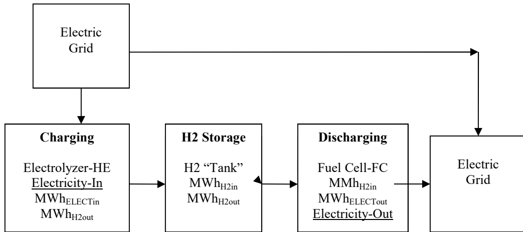
Schematic of H2 Storage Plant
